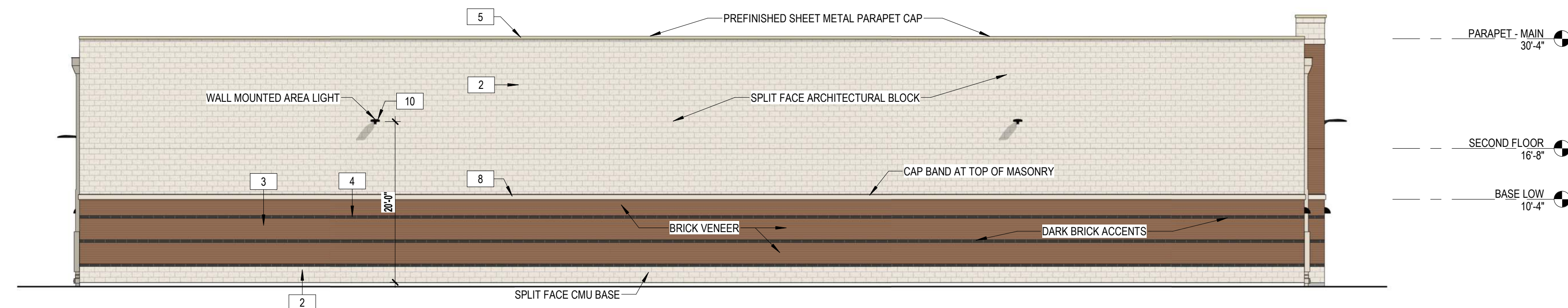
④ EAST ELEVATION (EASTWOOD MALL SIDE) 3/32" = 1'-0"
