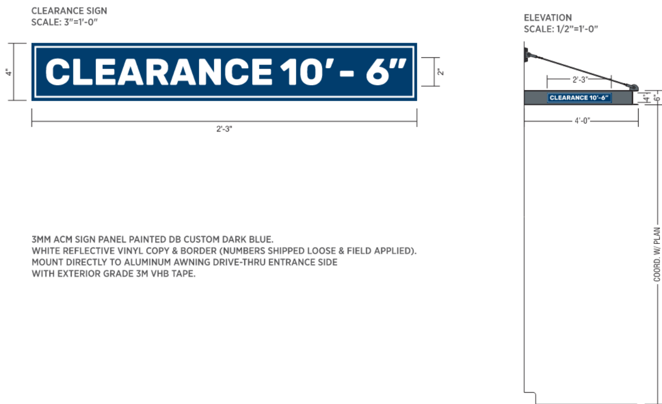
12 AWNING CLEARANCE SIGN, BY OTHERS AT DRIVE-THRU WINDOW - REFERENCE ONLY 12" = 1'-0"
