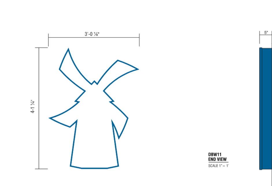
9 BUILDING SIGN, WINDMILL, BY OTHERS - REFERENCE ONLY 12" = 1'-0"
