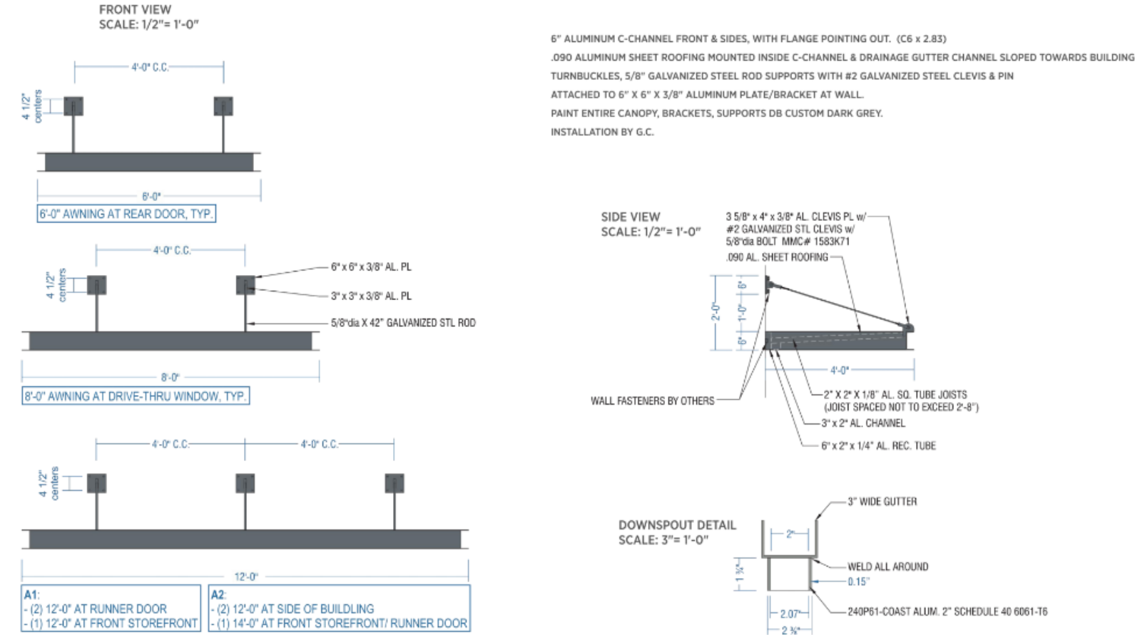
8 PRE-FAB. METAL AWNINGS, BY OTHERS - REFERENCE ONLY 12" = 1'-0"
