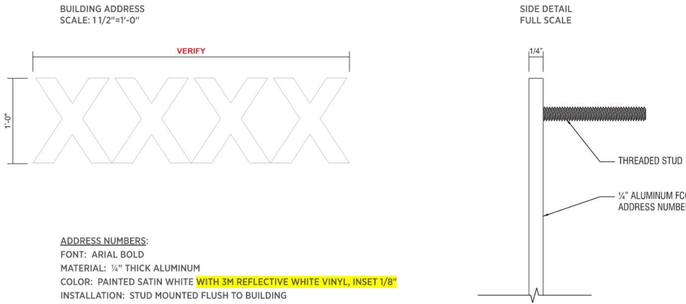
13 BUILDING ADDRESS NUMBERS BY OTHERS - REFERENCE ONLY 12" = 1'-0"
