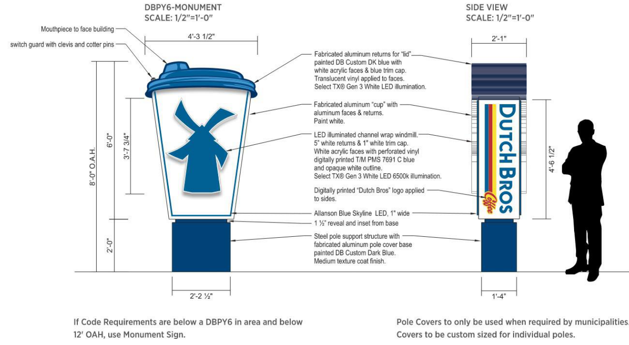
14 ILLUMINATED MONUMENT CUP SIGN 12" = 1'-0"
