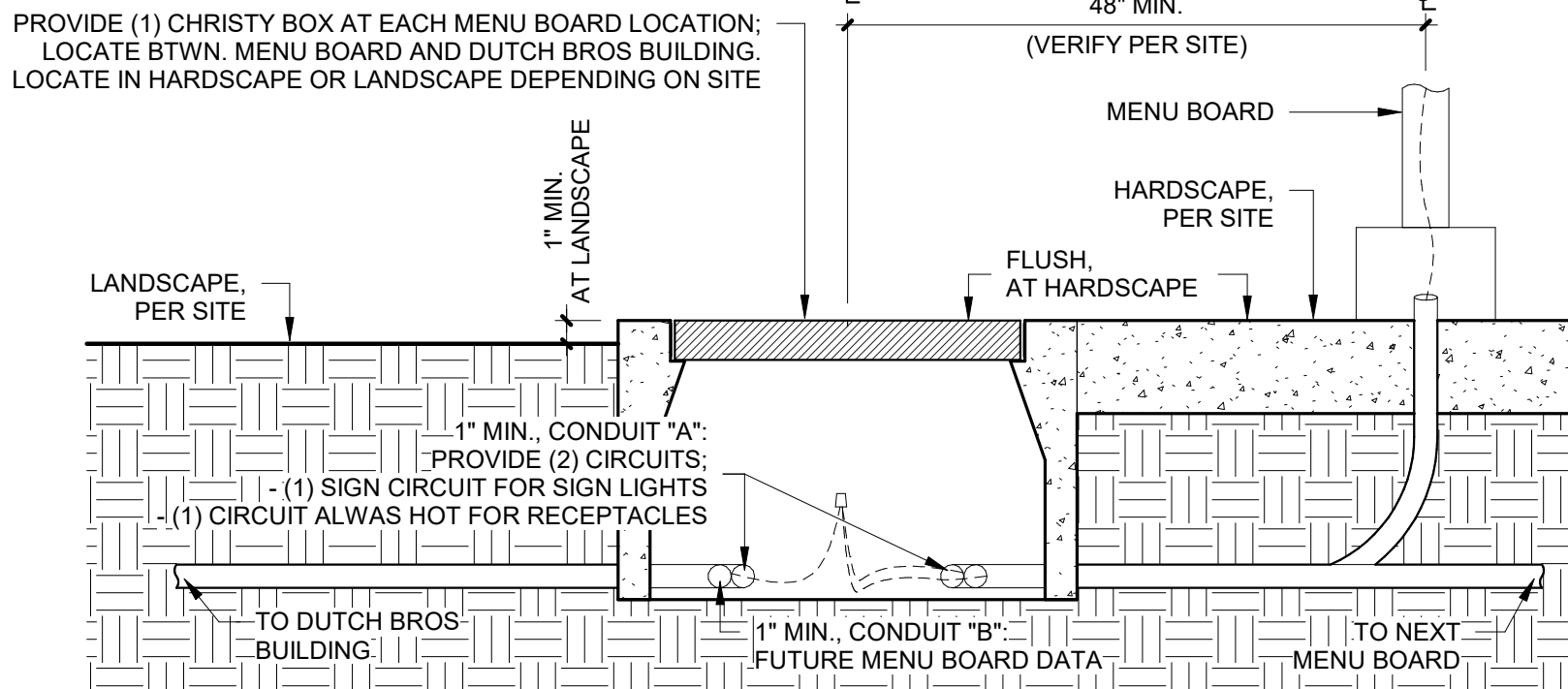
3 MENU BOARD & CHRISTY BOX - REFERENCE ONLY NTS
