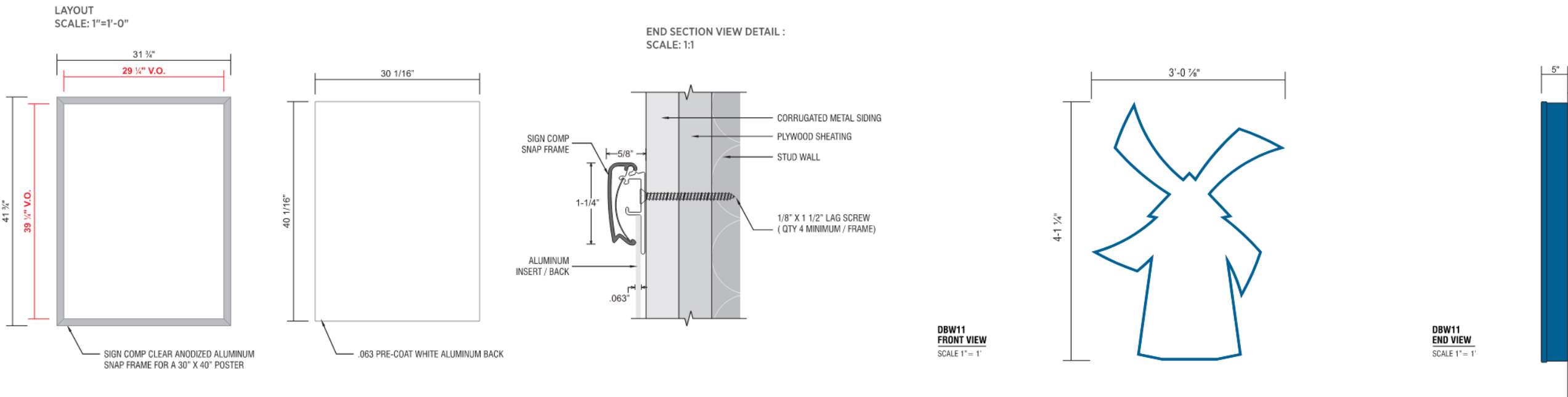
10 BUILDING SIGN, SNAP FRAMES, BY OTHERS - REFERENCE ONLY 12" = 1'-0"
