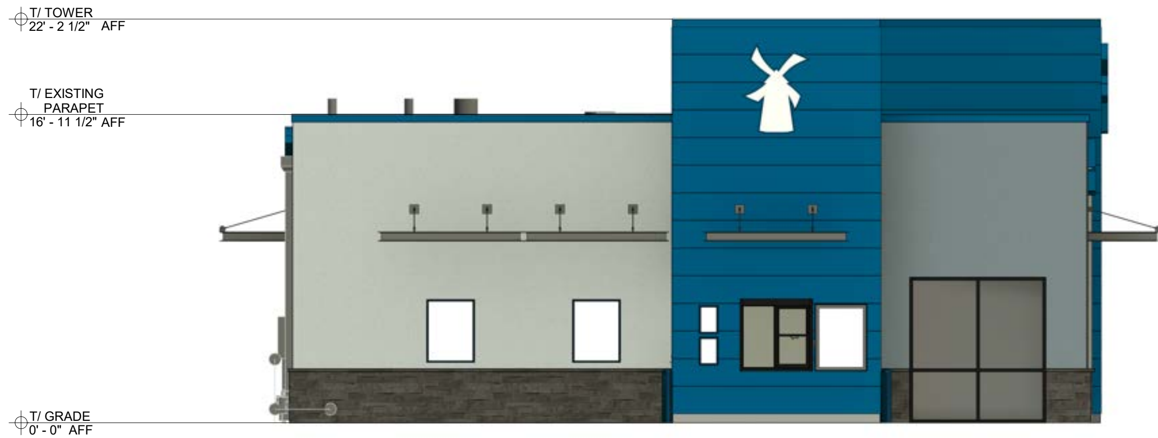
1 REC - EAST ELEVATION 3/16" = 1'-0"
