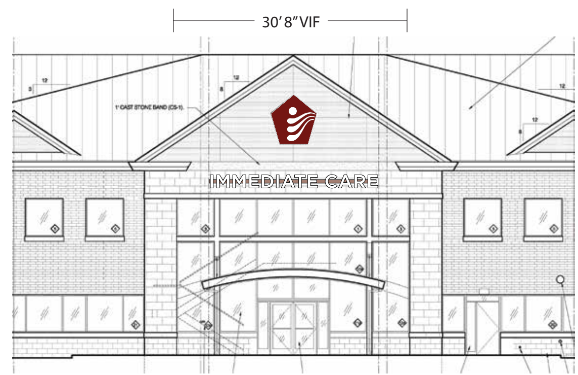
Proposed placement - North Elevation - NTS. See drawing A-201 for full scaled view.
