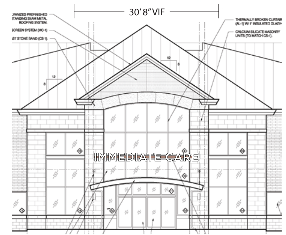
Proposed placement - South Elevation - NTS. See drawing A-201 for full scaled view.
